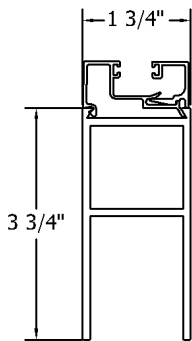
SINGLE ACTING
